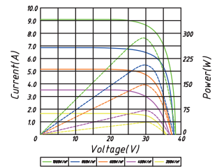
I-V CURVE TP660P Pm(W)260
